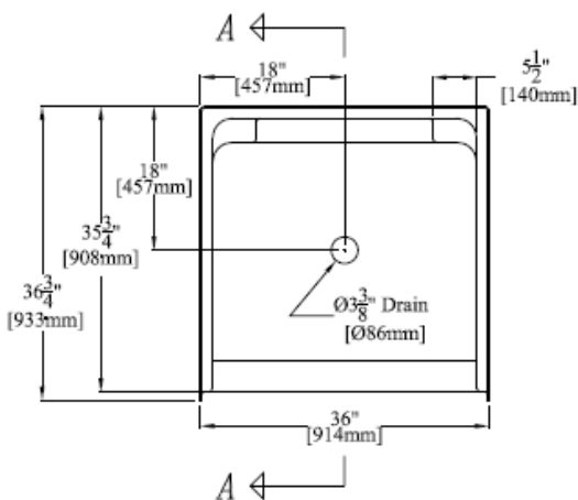
PLAN 36" [914mm] Shower w/ Molded Soap Ledges & Molded Foot Rest CENTER DRAIN
