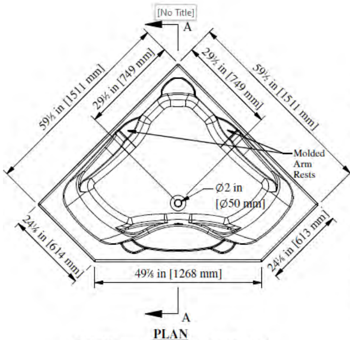
60" [1524mm] Acrylic Drop-In Bath tub w/ Molded Arm Rests
