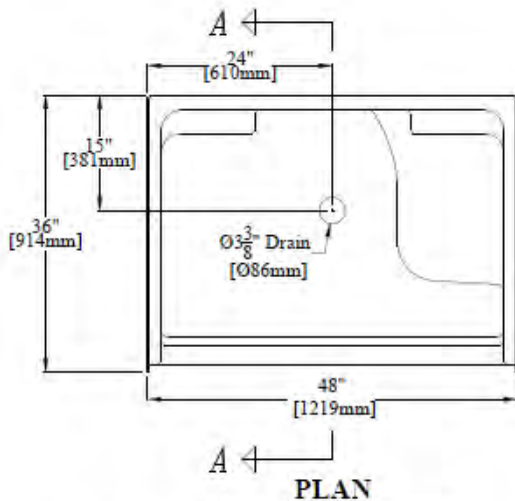
48" [1219mm] Shower w/ 6" [154mm] Threshold, Molded Seat
